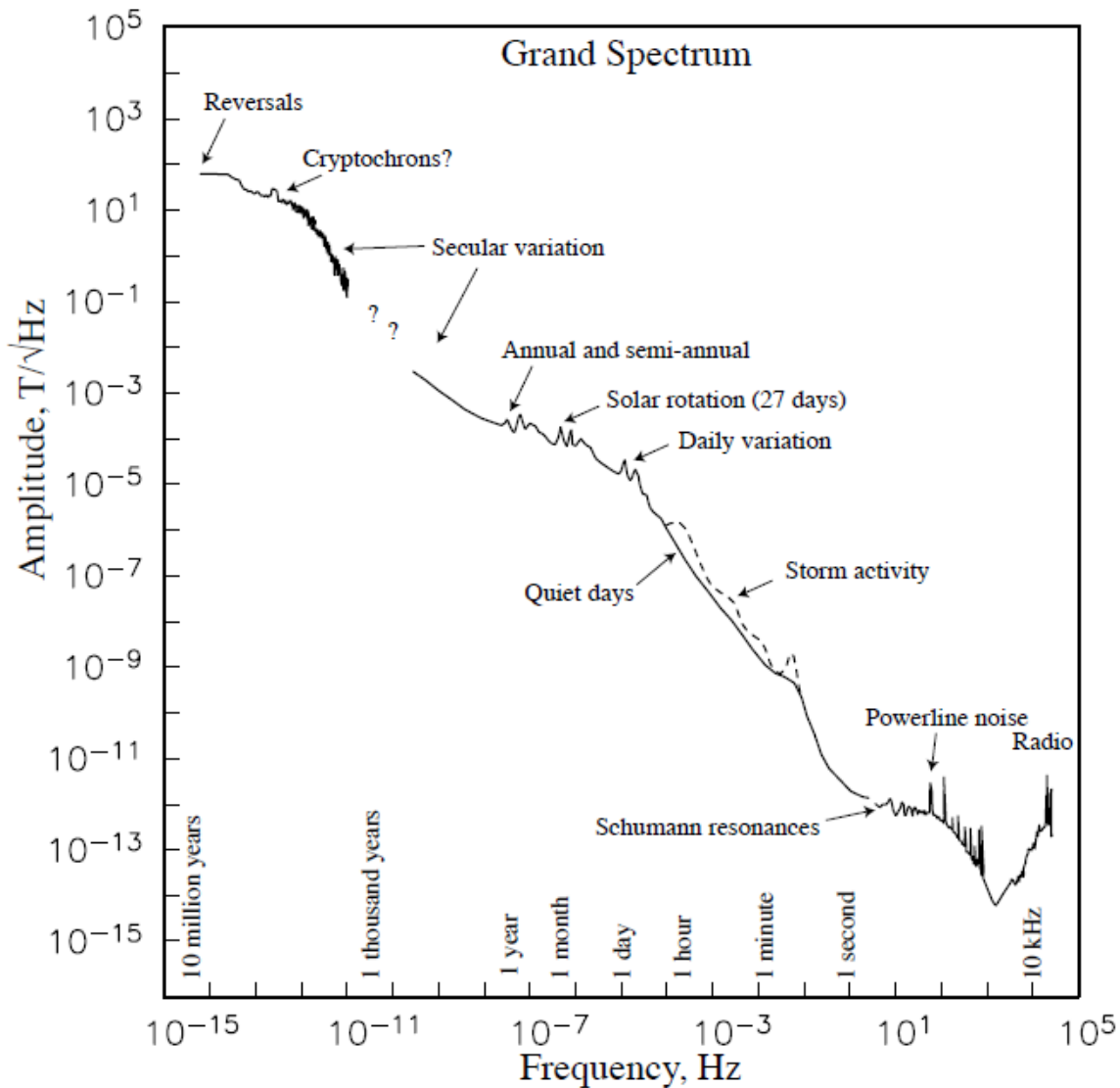
Figure 2: Composite amplitude spectrum of geomagnetic variations as a function of frequency (Constable and Constable, 2004): annotations indicate the predominant physical processes at the various timescales. Copyright American Geophysical Union, 2004, reproduced with their and the authors' permission.
