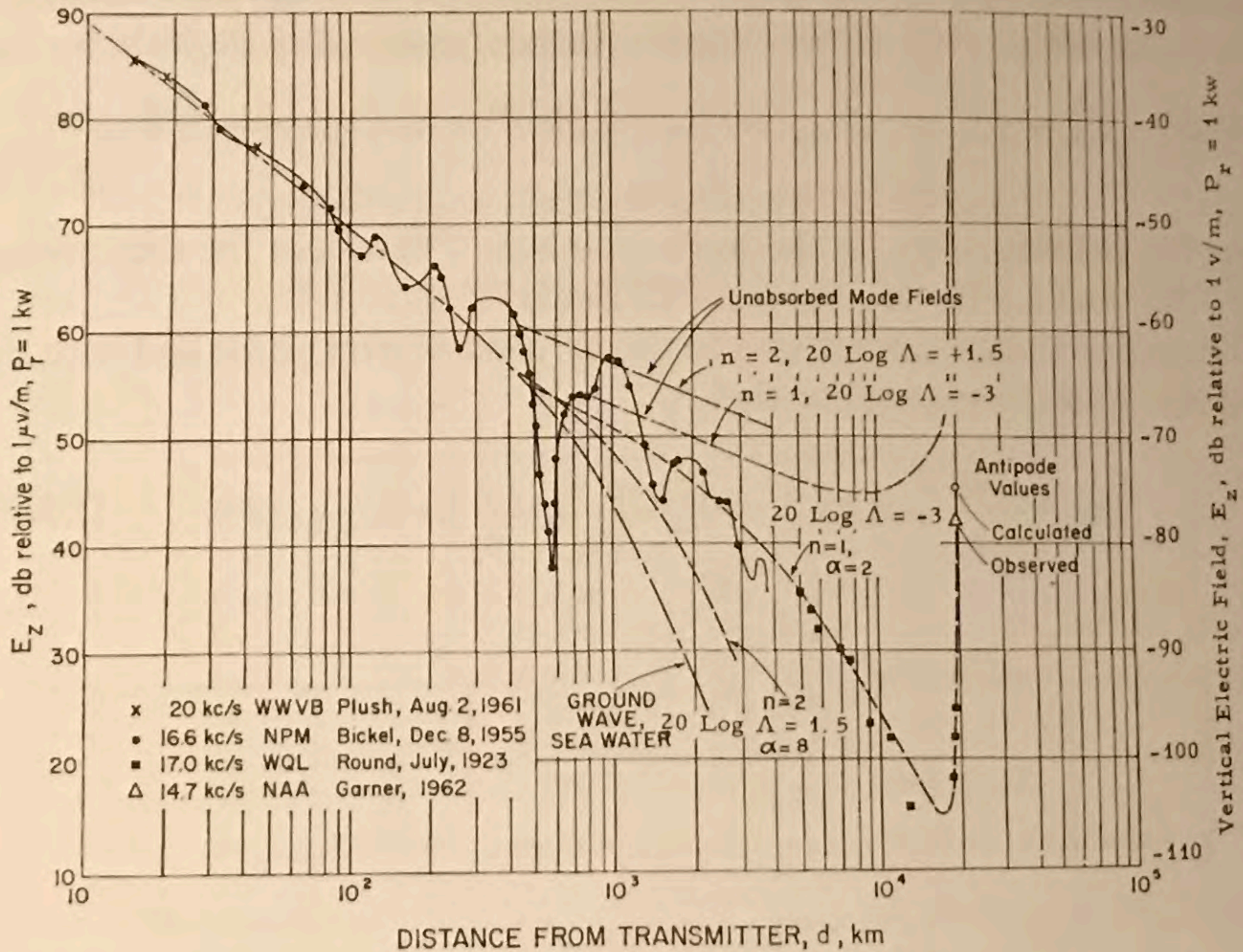
FIG. 3.5.55. Experimental and theoretical daytime field strength vs. distance.
