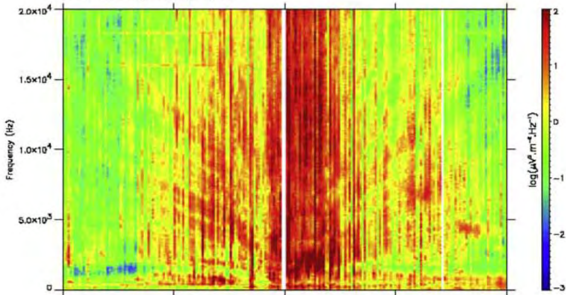
ICE VLF Spectrogram (onboard) E12
