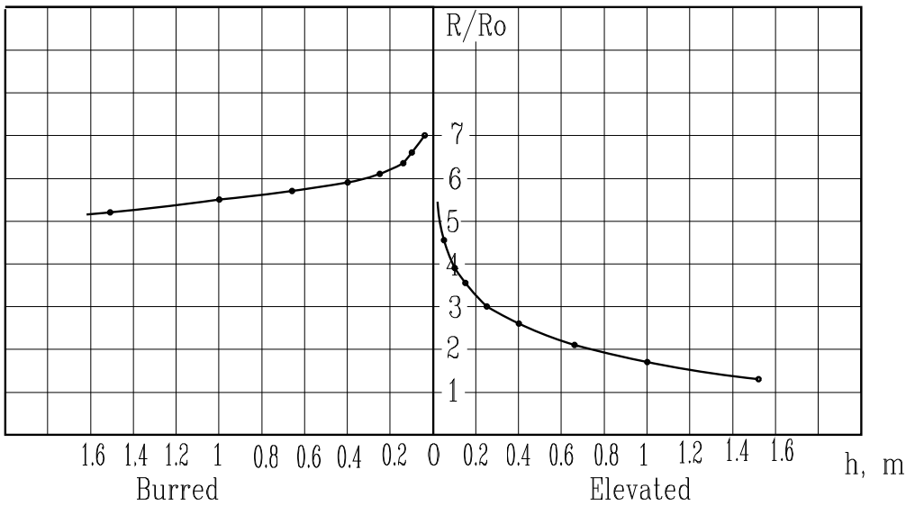
Ground loss for burred and elevated conterpoise H=20m r=1mm
